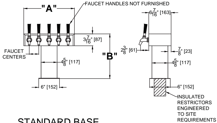
STANDARD BASE TEE TOWERS
